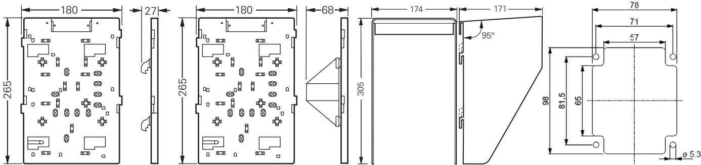
Mounting plate size 5 for wall/trellis mounting
