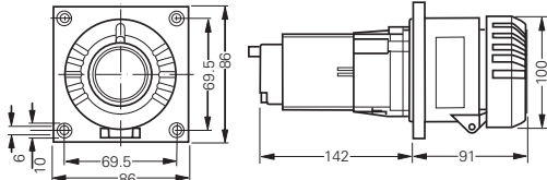
Flange socket 5-pole
