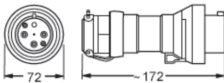
Plug 3-pole
